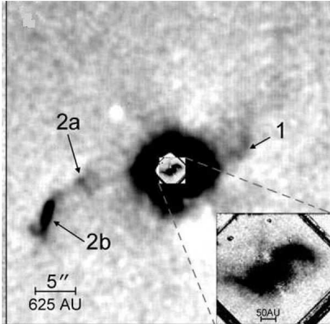
Figure 1: The inner 37'' \times 37'' continuum-subtracted, pure H 2 emission-line image of Elias 29 (Ybarra et al. 2006), with the K-band polarized intensity image of the inner 3'' \times 3'' in the inset (Huélamo et al. 2005). Figure produced by J. Ybarra (Univ. of Florida).
