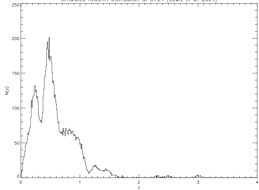
Simulated Redshift Distribution at B=24 (Cowie et al. 2004)
