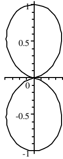
Non-relativistic
